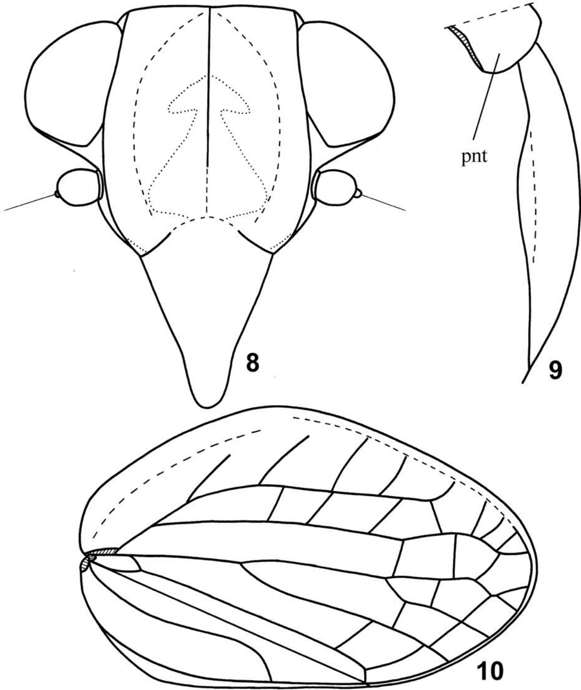
Figs 8–10. Granadus albirhombus gen. et sp. nov., male, paratype. 8 – head, frontal view, 9 – hypocostal plate of fore wing and paranotal lobe (pnt), 10 – fore wing.
