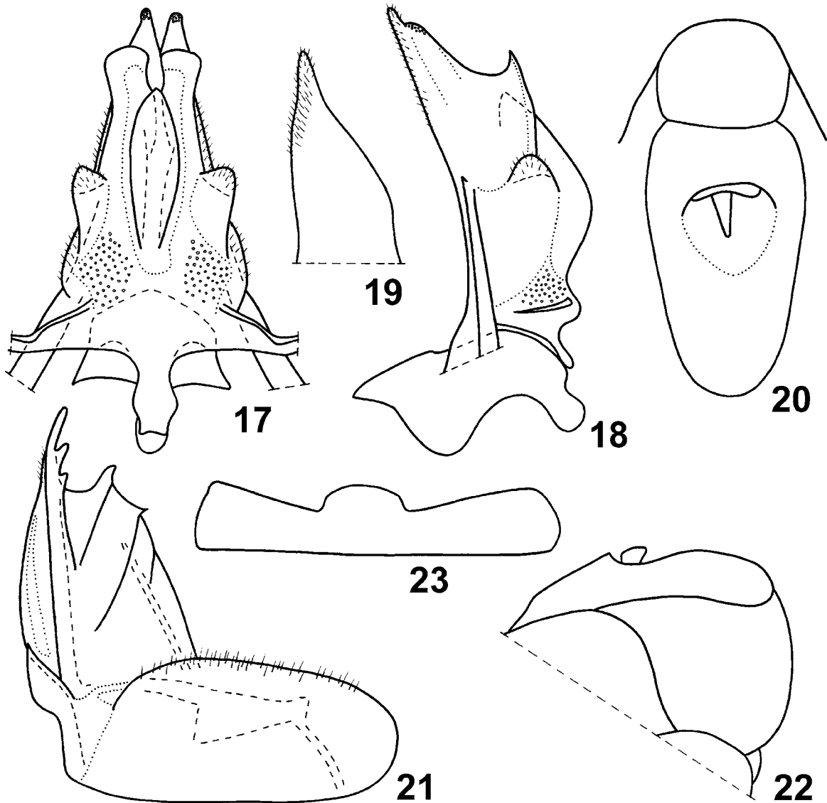
Figs 17–23. Granadus albirhombus gen. et sp. nov., paratype, female genitalia. 17 – posterior connective laminae of gonapophyses IX and gonospiculum bridge, dorsal view, 18 – same, lateral view, 19 – endogonocoxal process, 20 – anal tube, dorsal view, 21 – anterior connective lamina of gonapophyse VIII, lateral view, 22 – gonoplacs and anal tube, lateral view, 23 – sternite VII, ventral view.
